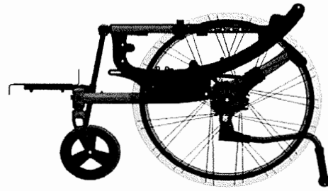
Anti tip tube, flip up
